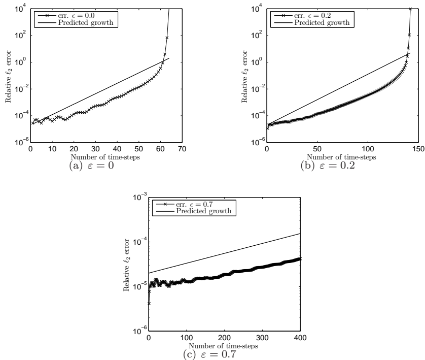
FIGURE 15. Relative \ell_2 error in the RBF solution of the geopotential height for the steady state test case together with the predicted growth rate from equation 18. The value of \varepsilon used is given below each figure. For all plots, \Delta t = 1080 s and N = 484 .
