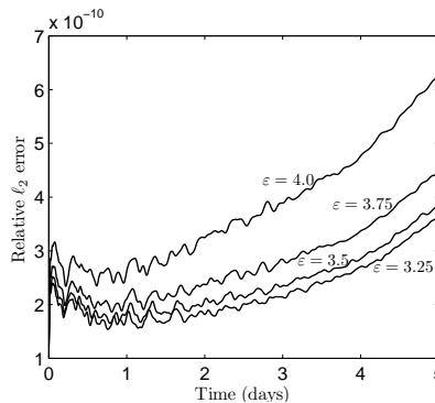
FIGURE 10. Relative l_2 errors in the height field for the steady state test case as a function of time and different values of \varepsilon .
