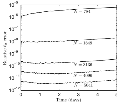
FIGURE 7. Relative \ell_2 error in the height field for the steady state test case as a function of time and N . \varepsilon = 3.25 for all N .
