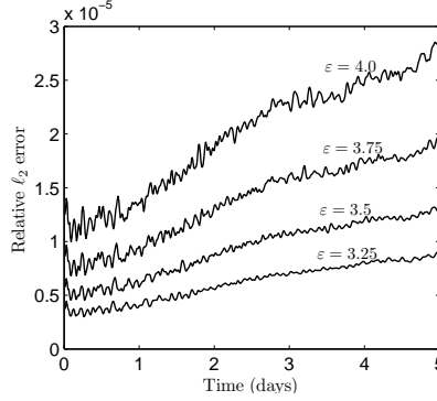
FIGURE 21. Relative \ell_2 errors in the height field for the unsteady flow test case with N = 3136 as a function of time and different values of the shape parameter \varepsilon .
