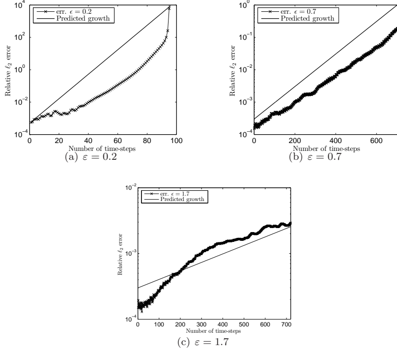
FIGURE 23. Relative \ell_2 error of the height field for the unsteady test case together with the predicted growth rate from equation 18. \Delta t = 1200 s (20 min) and N = 1849 . The value of \epsilon used is indicated below each figure. Figures (b) and (c) are run for 720 time steps, corresponding to 10 days of integration.
