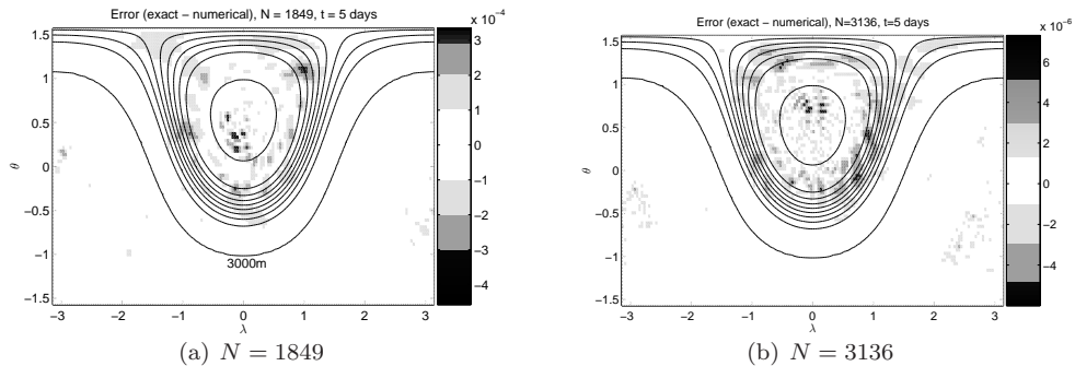
FIGURE 6. The error (exact - numerical) for the height field from the steady state test case at t = 5 days on an “unrolled” sphere. (a) N = 1849 nodes, (b) N = 3136 nodes. Solid black lines correspond to contours of the exact solution plotted from 2100m to 3000m in increments of 100m. \varepsilon = 3.25 for all N .
