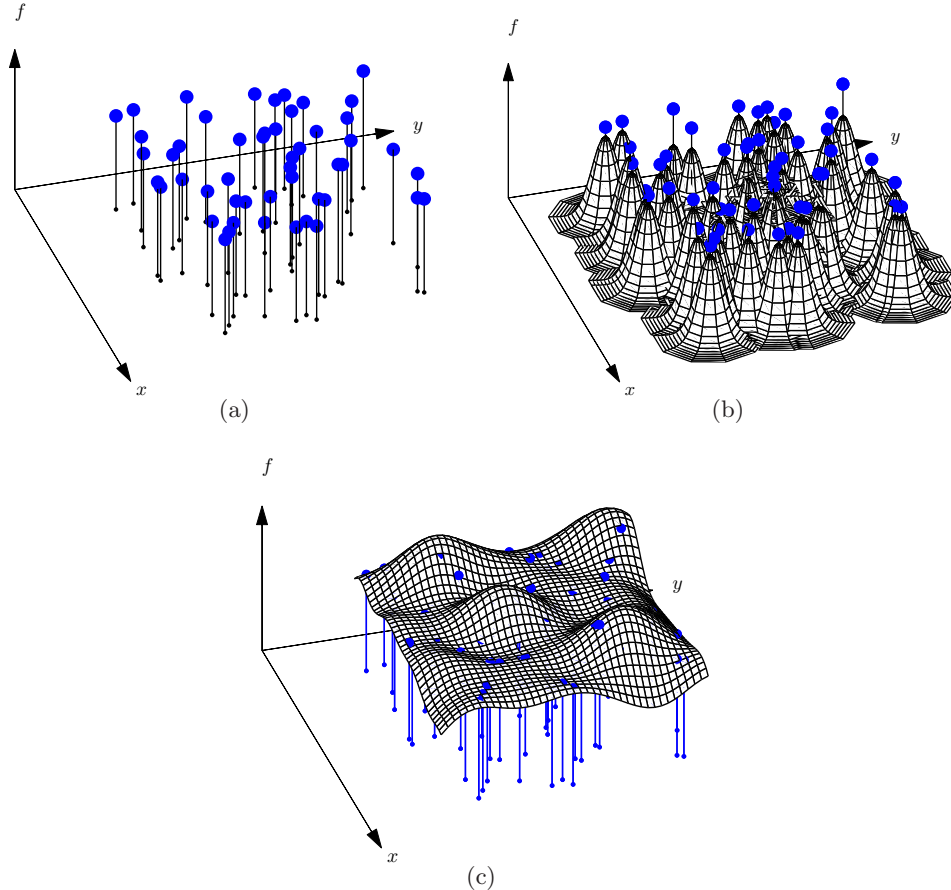
Figure 1: (a) Data values \{f_j\}_{j=1}^N , (b) the RBF collocation functions, (c) the resulting RBF interpolant.
