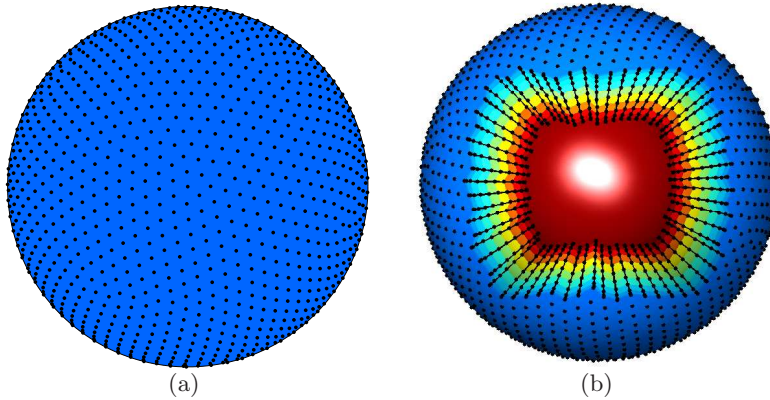
Figure 2: (a) RBF node layout on the surface of a sphere; (b) 3D view of the discretization of the spherical shell used in the hybrid RBF-PS calculation. Blue is the outer boundary and red is the inner boundary, black circles display the computational nodes, which are distributed in the radial direction along the extrema of the Chebyshev polynomials. Note the spherical shell has been opened up in (b) to show the detail.
