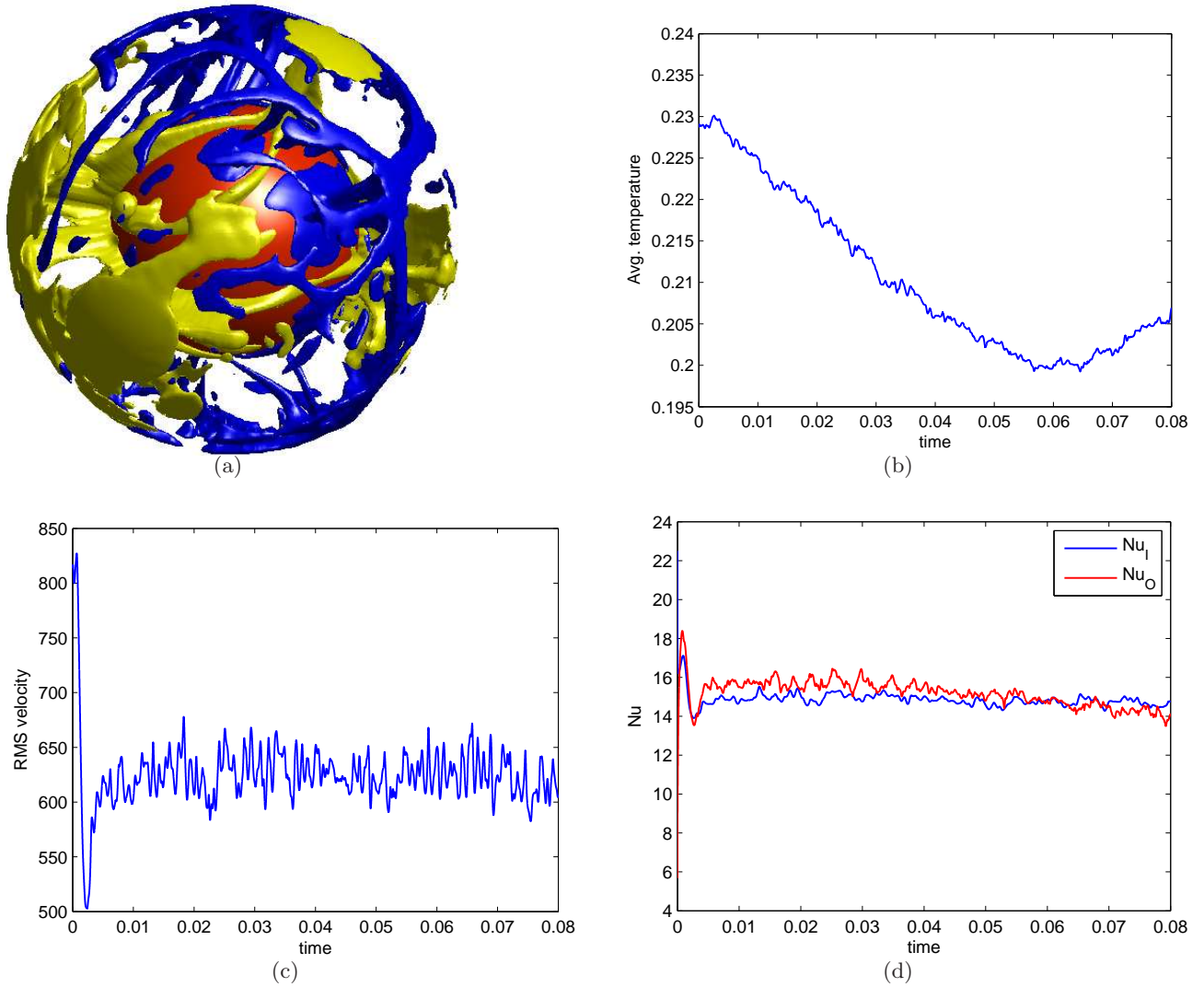
Figure 7: Results for Ra = 10^6 test case: (a) Residual temperature, \delta T , at t = 0.08 , where yellow corresponds to \delta T = 0.1 , blue corresponds to \delta T = -0.1 , and the red solid sphere shows the inner boundary of the 3D shell corresponding to the core; (b) Average temperature, \langle T \rangle , vs. time; (c) Average RMS velocity, \langle V_{\text{rms}} \rangle , vs. time; (d) Inner and outer Nusselt numbers, Nu_i and Nu_o , vs. time.
