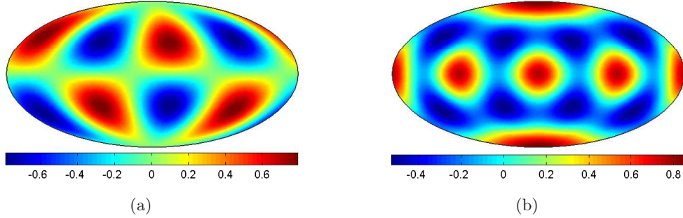
Figure 3: \theta - \lambda dependence of the initial condition for the (a) Tetrahedral and (b) Cubic mantle convection test cases.
