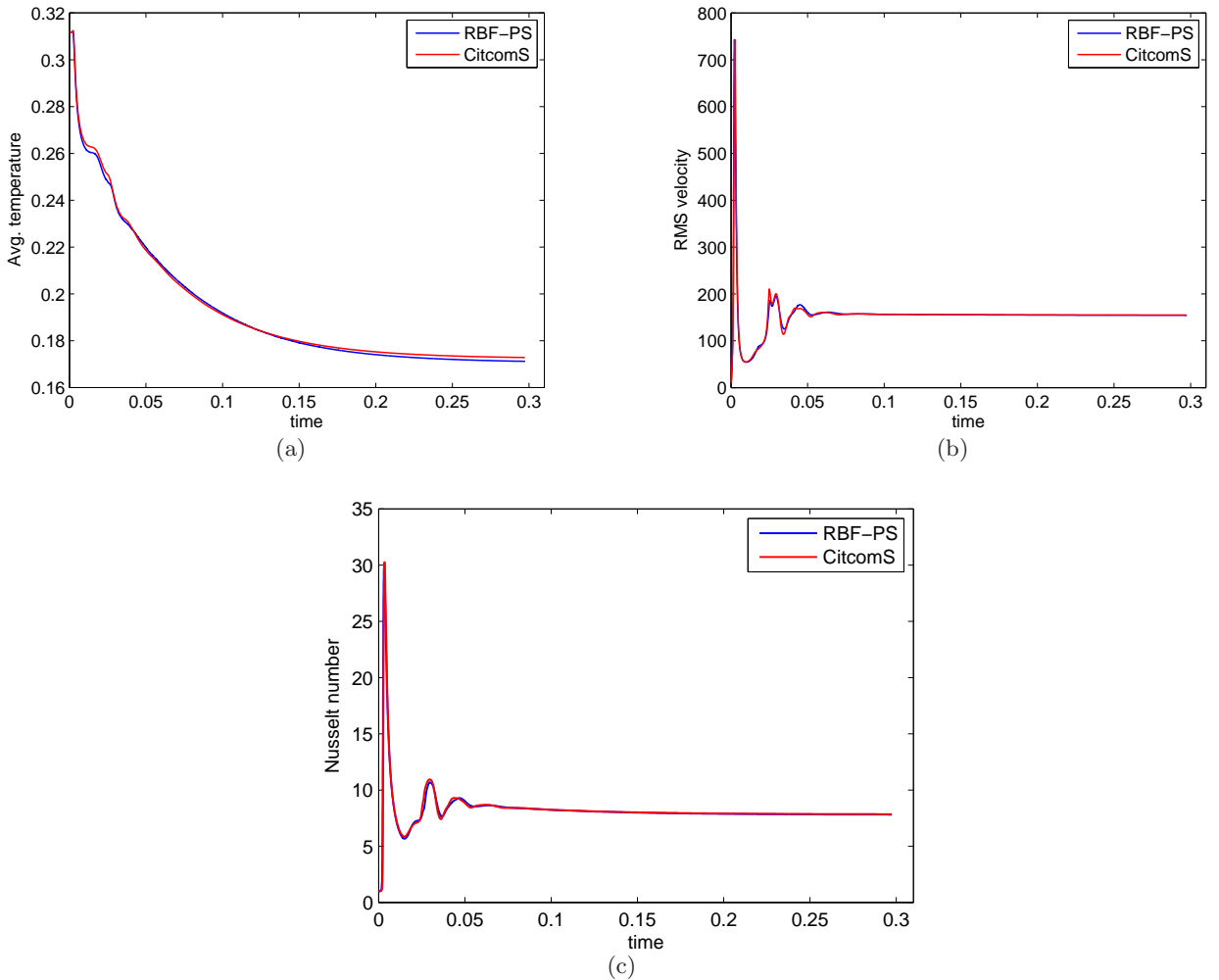
Figure 6: Time plots of the (a) \langle T \rangle , (b) \langle V_{\text{rms}} \rangle , and (c) \text{Nu}_o , comparing the results (obtained through CIG) of the CitcomS and RBF-PS for isoviscous mantle convection at \text{Ra} = 10^5 .
