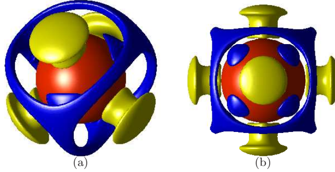
Figure 4: Steady-state isosurfaces of the residual temperature, \delta T , at t = 1 for the isoviscous (a) Tetrahedral and (b) Cubic mantle convection test cases at Ra = 7000 computed with the RBF-PS model. Yellow corresponds to \delta T = 0.15 and denotes upwelling relative to the average temperature at each radial level, while blue corresponds to \delta T = -0.15 and denotes downwelling. The red solid sphere shows the inner boundary of the 3D shell corresponding to the core.
