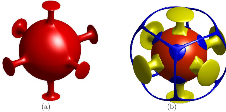
Figure 5: (a) Steady-state isosurface temperature T = 0.5 at time t = 0.3 . (b) Steady-state isosurface of the residual temperature, \delta T = T(r, \lambda, \theta) - \langle T(r) \rangle , at t = 0.3 for the isoviscous cubic mantle convection test case at Ra = 10^5 computed with the RBF-PS model. The same color scheme as Figure 4 has been applied.
